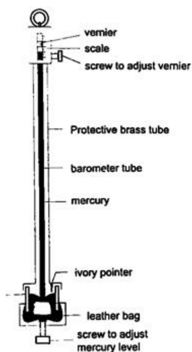
Fortin barometer
